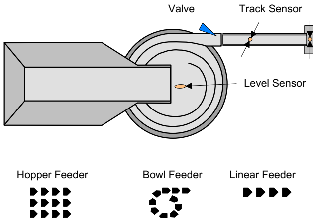
Feed Station with Bowl, Linear and Hopper feeders
